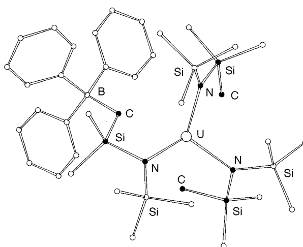
Fig. 1 Structure of [U\{N(SiMe_3)_2\}_2\{N(SiMe_3)_2SiMe_2CH_2B(C_6F_5)_3\}] in the crystal. All black atoms co-ordinate the uranium atom by strong covalent (N) or weaker multicentre bonds (Si, C). All hydrogen and fluorine atoms are omitted for clarity
