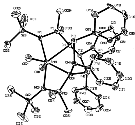
Figure 1. Molecular structure of 3 shown with 30% thermal ellipsoids. Selected bond lengths (Å) and angles (deg): Zr(1)–C(1) 2.425(8), Zr(1)–C(3) 2.427(9), Zr(1)–N(1) 2.249(7), Zr(1)–N(2) 2.256(7), Zr(1)–Cl(1) 2.461(3), Zr(1)–Cl(2) 2.428(3), Cl(1)–Zr(1)–Cl(2) 133.01(10), C(1)–Zr(1)–N(1) 68.3(3), C(3)–Zr(1)–N(2) 67.7(3), N(1)–Zr(1)–N(2) 158.1(3), C(1)–Zr(1)–C(3) 68.0(3).
