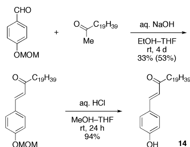
Chart 5. Synthesis of a Ketone-Derivative
