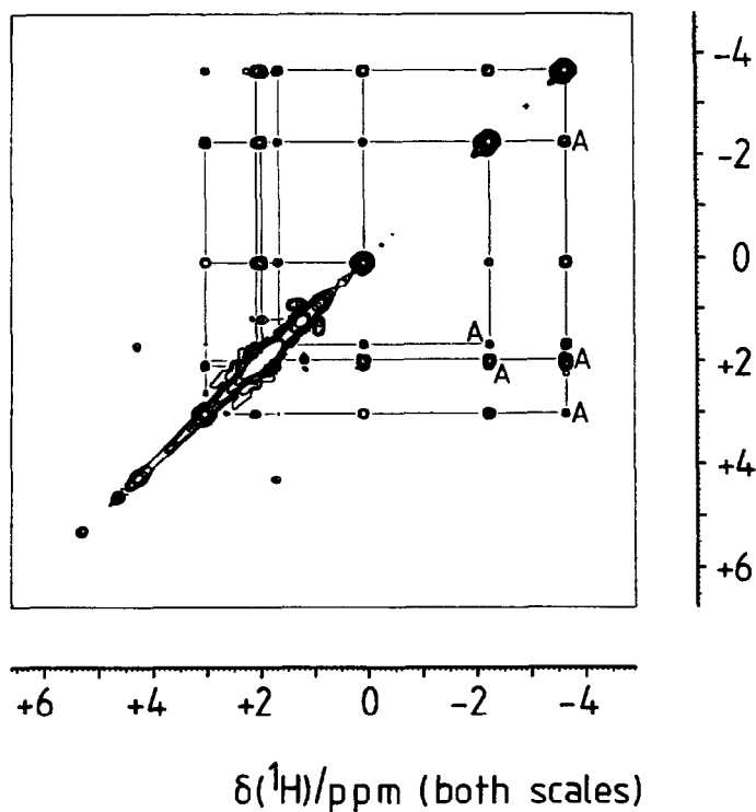
Fig. 3. A 2D [ ^1\text{H} - ^1\text{H} ]-COSY NMR contour plot for a sample of compound 3 in \text{CDCl}_3 solution at ca. 304 K, recorded under conditions of \{^{11}\text{B} (broad band noise) \} decoupling. The ^1\text{H} resonance of BH(6) at \delta +6.27 was insufficiently decoupled to appear on the plot, and ^1\text{H} (5,6) (off-scale at -17.51 ppm) did not exhibit any cross-peaks with the other proton resonances. Correlations arising from ^2J(^1\text{H}-\text{B}-^1\text{H}) paths (designated A) are on the lower right-hand diagonal half; the other correlations arise from ^3J(^1\text{H}-\text{B}-\text{B}-^1\text{H}) .
