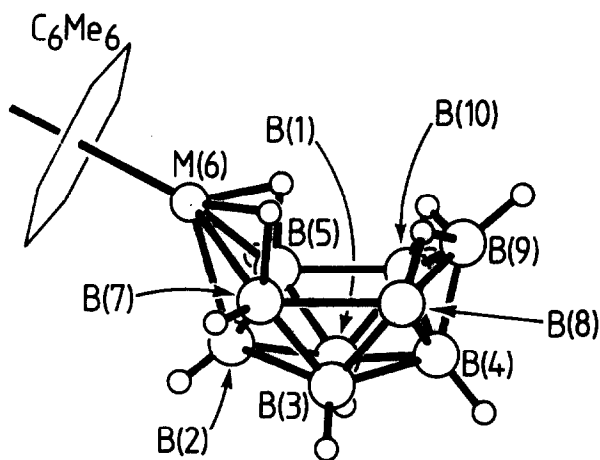
Fig. 1. Proposed molecular structure of [6(\eta^6\text{-C}_6\text{Me}_6)\text{-nido-6-MB}_9\text{H}_{13}] , where M = \text{Ru} (compound 1), \text{Os} (compound 2).
