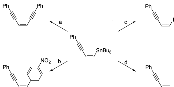
Scheme 12. (a) \text{PhC}\equiv\text{CBr} (0.92 equivalents), \text{Pd}_2(\text{dba})_3 , (2-furyl) _3\text{P} (5 mol% of Pd, \text{Pd}/(2\text{-furyl})_3\text{P} = 1/4 ), NMP, 50°C, 18 h, 58% (based on \text{PhC}\equiv\text{CBr} ). (b) 4- \text{O}_2\text{NC}_6\text{H}_4\text{I} (0.92 equivalents), \text{Pd}_2(\text{dba})_3 , (2-furyl) _3\text{P} (5 mol% of Pd, \text{Pd}/(2\text{-furyl})_3\text{P} = 1/4 , toluene, 90°C, 13 h, 85% (based on 4- \text{O}_2\text{NC}_6\text{H}_4\text{I} ). (c) \text{I}_2 (1.4 equivalents), THF, 0°C, 40 min, 92%. (d) Conc. HCl, THF, r.t., 1 h, 81%.
