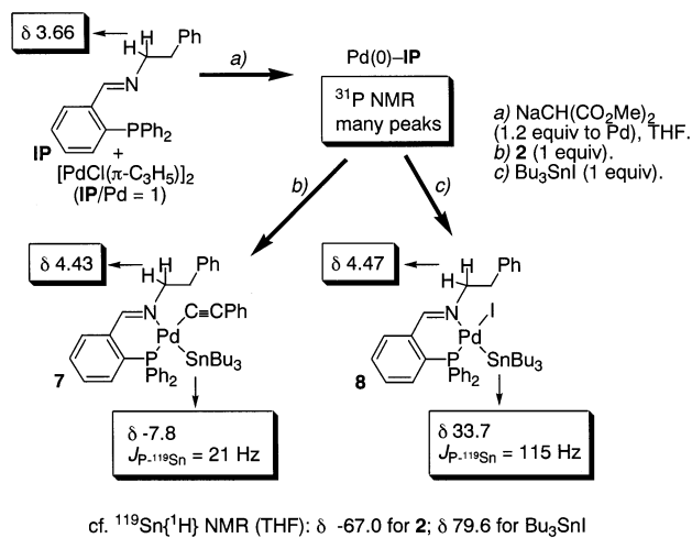
Fig. 3. ^{31}\text{P}\{^1\text{H}\} -, ^{119}\text{Sn}\{^1\text{H}\} - and ^1\text{H} -NMR (THF- d_8 ) parameters (chemical shift and J_{\text{Sn-P}} ) of \text{Pd(0)/IP} and its reaction products with 2 or \text{Bu}_3\text{SnI} .
