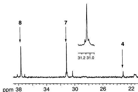
Fig. 2. ^{31}\text{P}\{^1\text{H}\} -NMR (109 MHz) spectrum of the reaction mixture (at 2–33% conversion) of [\text{PdCl}(\pi\text{-C}_3\text{H}_5)]_2 -IP catalyzed coupling of 2 with 1 in THF.
