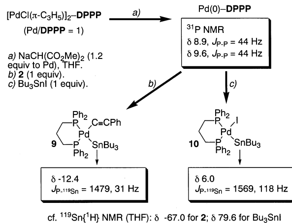
Fig. 4. ^{31}\text{P}\{^1\text{H}\} -, ^{119}\text{Sn}\{^1\text{H}\} - and ^1\text{H} -NMR (THF) parameters (chemical shift, J_{\text{Sn-P}} and J_{\text{P-P}} ) of \text{Pd(0)/DPPP} and its reaction products with 2 or \text{Bu}_3\text{SnI} .
