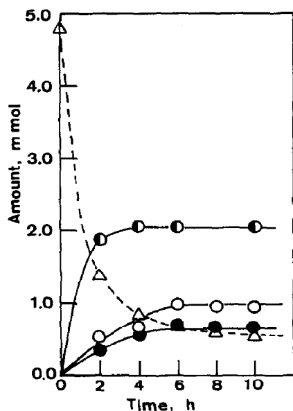
Fig. 2. Oxidation of cyclohexene with t-BuOOH catalyzed by cluster 1 in 1,2-dichloroethane (10 cm 3 ) at 70 °C. Catalyst, 6.0 \times 10^{-2} mmol; cyclohexene, 4.8 mmol (initial amount); t-BuOOH, 12.0 mmol (initial amount); ●, 2-cyclohexen-1-yl t-butylperoxide; ○, 2-cyclohexen-1-one; ●, 1,2-epoxycyclohexane; Δ, cyclohexene.
