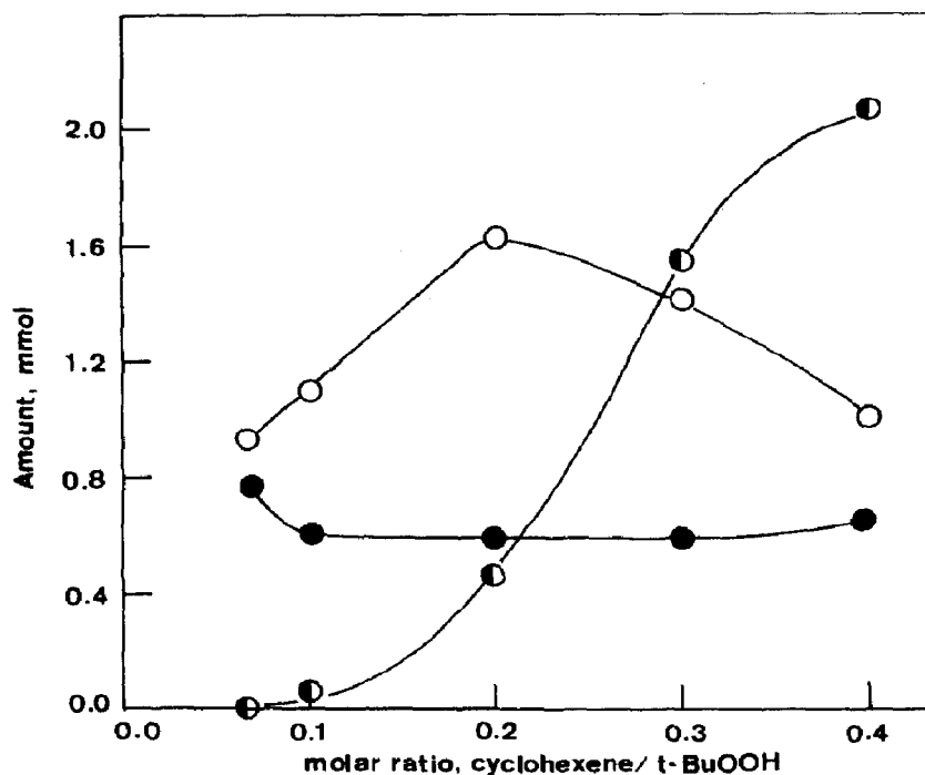
Fig. 3. Effect of the t-BuOOH concentration on the yield of each product after 5 h of the reaction of cyclohexene with t-BuOOH catalyzed by cluster 1 in 1,2-dichloroethane (10 cm 3 ) at 70 °C. Catalyst, 6.0 \times 10^{-2} mmol; cyclohexene, 4.8 mmol (initial amount). Symbols are the same as those in Fig. 2.
