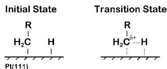
Figure 10. Transition state for alkyl group hydrogenation on the Pt(111) surface. The substituent effects reveal that the transition state is relatively cationic with respect to the initial state and that the transition state holds a higher charge density.
