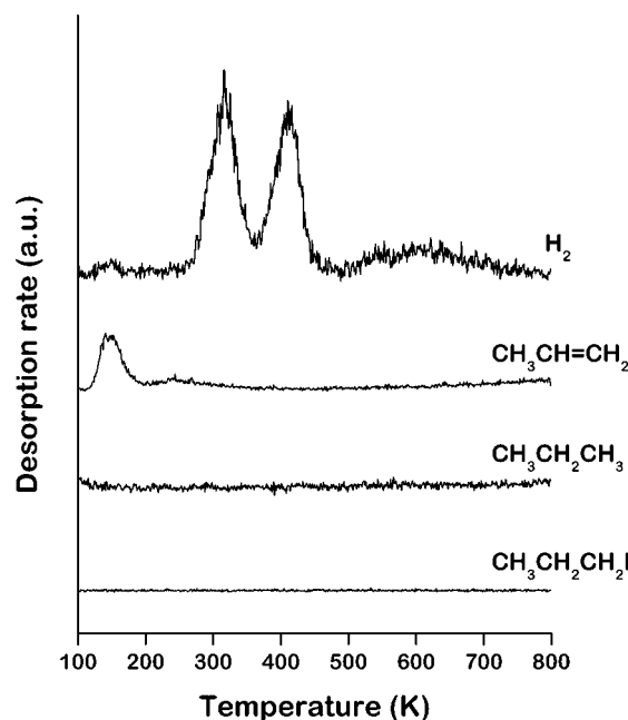
Figure 3. TPR spectra of 1.5 L CH 3 CH 2 CH 2 I on clean Pt(111). The surface was exposed to CH 3 CH 2 CH 2 I at 95 K. The heating rate was 2 K/s. Signals were monitored at m/q = 2, 27, 29 , and 127. No production of propane is observed.
