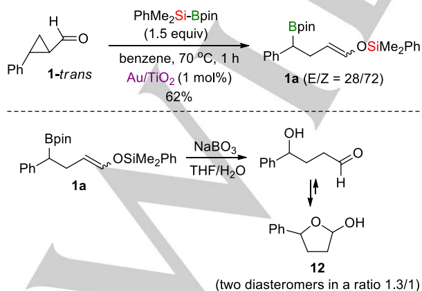
Scheme 5. Possible mechanisms for the formation of rearranged silaboration product 1a .
