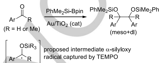
Scheme 1. Reaction of silylborane pinB-SiMe 2 Ph with aromatic carbonyl compounds catalyzed by Au/TiO 2 , and the proposed intermediate \alpha -silyloxy radical. [6]
