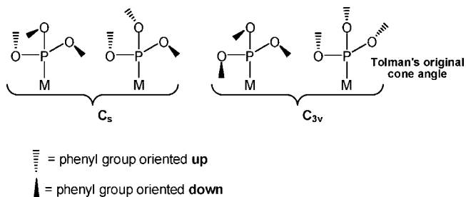
Figure 2. Conformers of P(OPh) 3 .
