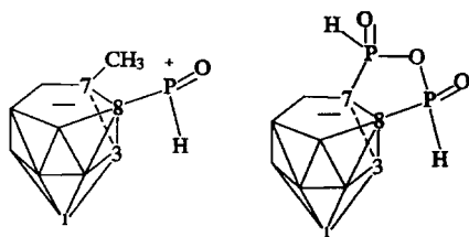
Fig. 4. Proposed structures of nido -carboranylmmono- and -bis(ethoxyphosphines).
