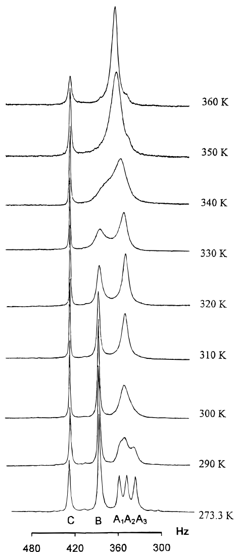
Figure 9. Variable temperature 300 MHz ^1\text{H} NMR spectra of the tert -butyl region of a mixture of trans - 10 ( A_1 , A_2 , A_3 ), cis - 10 ( B ), and \text{H}_2\text{9} ( C ) in \text{D}_2\text{O} (pD 12.1). [ 10 ] = 0.015 M. [ \text{H}_2\text{9} ] = 0.008 M.
