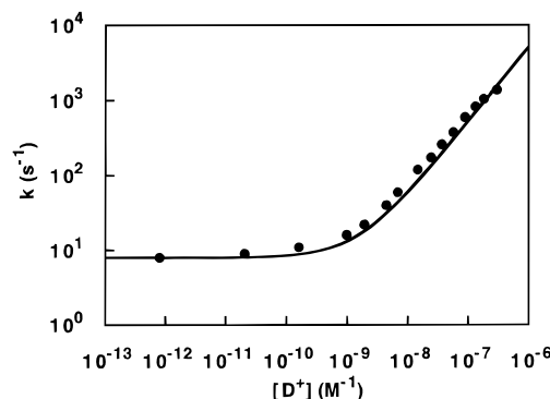
Figure 4. pD dependence of the rate constants for the interconversion of the enantiomers of 4 in D_2O (circles). Rate constants were obtained by line-shape analysis of the experimental spectra (isopropyl methyl proton region) recorded in buffered D_2O solutions at 298 K (5% phosphate buffer; 4 ] = 0.015 M). The rate constants were fit to the equation k = k_0 + k_1[D^+] by least-squares methods ( k_0 = 9.0(6) \text{ s}^{-1} , k_1 = 6.4(2) \times 10^9 \text{ M}^{-1} \text{ s}^{-1} ).
