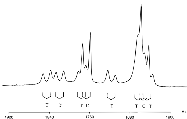
Figure 8. Experimental 400 MHz ^1\text{H} NMR spectrum of 10 (benzylic proton region) in \text{DMSO-}d_6 after irradiation in the benzyl proton region at 298 K. C and T denote the AB spin systems of cis-10 and trans-10 , respectively.
