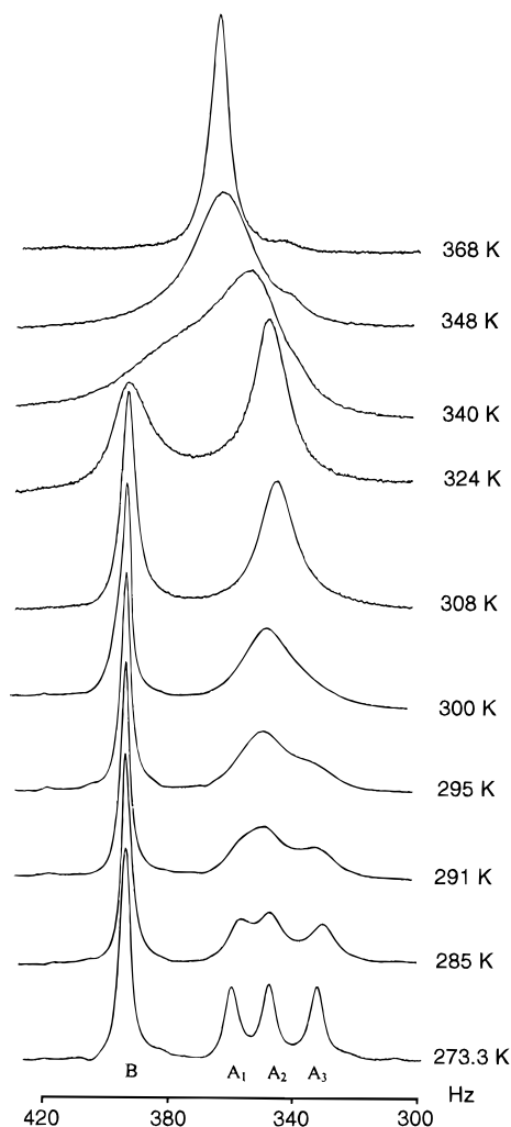
Figure 6. Variable temperature 300 MHz ^1\text{H} NMR spectra of the tert -butyl region of cis - 10 (B) and trans - 10 ( A_1 , A_2 , A_3 ) in \text{D}_2\text{O} (pD 9.8). [\text{10}] = 0.015 \text{ M} .
