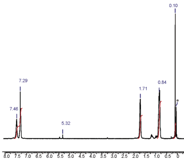
Figure 1. ^1\text{H} NMR spectrum of (\text{Et}_2\text{PhP})_3\text{AgSSiMe}_3 in \text{CD}_2\text{Cl}_2 at -70^\circ\text{C} . The asterisk indicates silicone grease.
