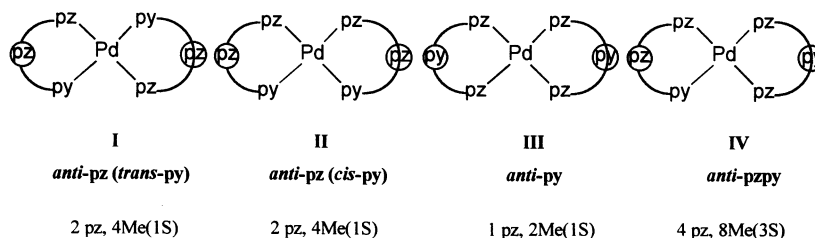
Scheme 6. Possible anti coordination isomers of 6b .
