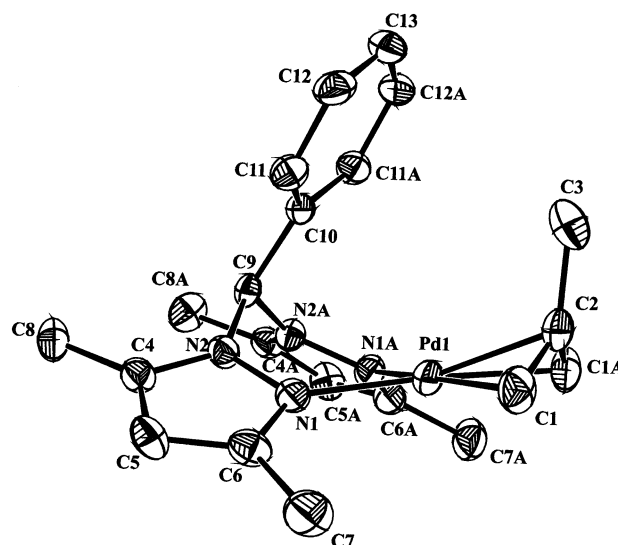
Fig. 1. Molecular structure of the cation of complex 5aM .
