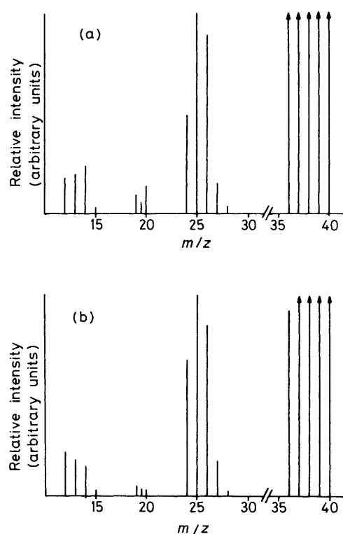
Figure 2. CA spectra of the EI induced fragment ions with m/z 40 from but-3-ynoic acid (a) and buta-2,3-dienoic acid (b)
