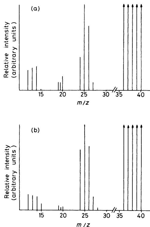
Figure 1. CA spectra of the molecular ions of allene (a) and propyne (b)
