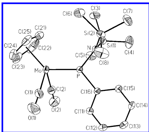
Figure 1. Molecular geometry and atom-labeling scheme for \text{Cp}(\text{CO})_2\text{Mo}\{\text{P}(\text{Ph})[\text{N}(\text{SiMe}_3)_2]\} ( 4a ) with H atoms omitted. Thermal ellipsoids are represented at the 25% probability level.
