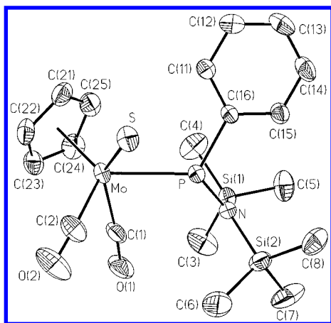
Figure 2. Molecular geometry and atom-labeling scheme for \text{Cp}(\text{CO})_2(\text{S})\text{Mo}\{\text{P}(\text{Ph})[\text{N}(\text{SiMe}_3)_2]\} ( 7a ) with H atoms omitted. Thermal ellipsoids are represented at the 25% probability level.
