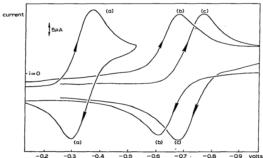
Fig. 2. 100 mV/s cyclic voltammograms of \sim 10^{-3} M (a) (\text{C}_6\text{H}_5\text{Cl})_2\text{Cr}^+ (b) (\text{C}_6\text{H}_5\text{C}_6\text{H}_5)_2\text{Cr}^+ (c) (\text{C}_6\text{H}_5\text{OCH}_3)_2\text{Cr}^+ in DMSO/0.1 M \text{Bu}_4\text{NClO}_4 at Pt electrode vs. SCE ( 25^\circ\text{C} ).
