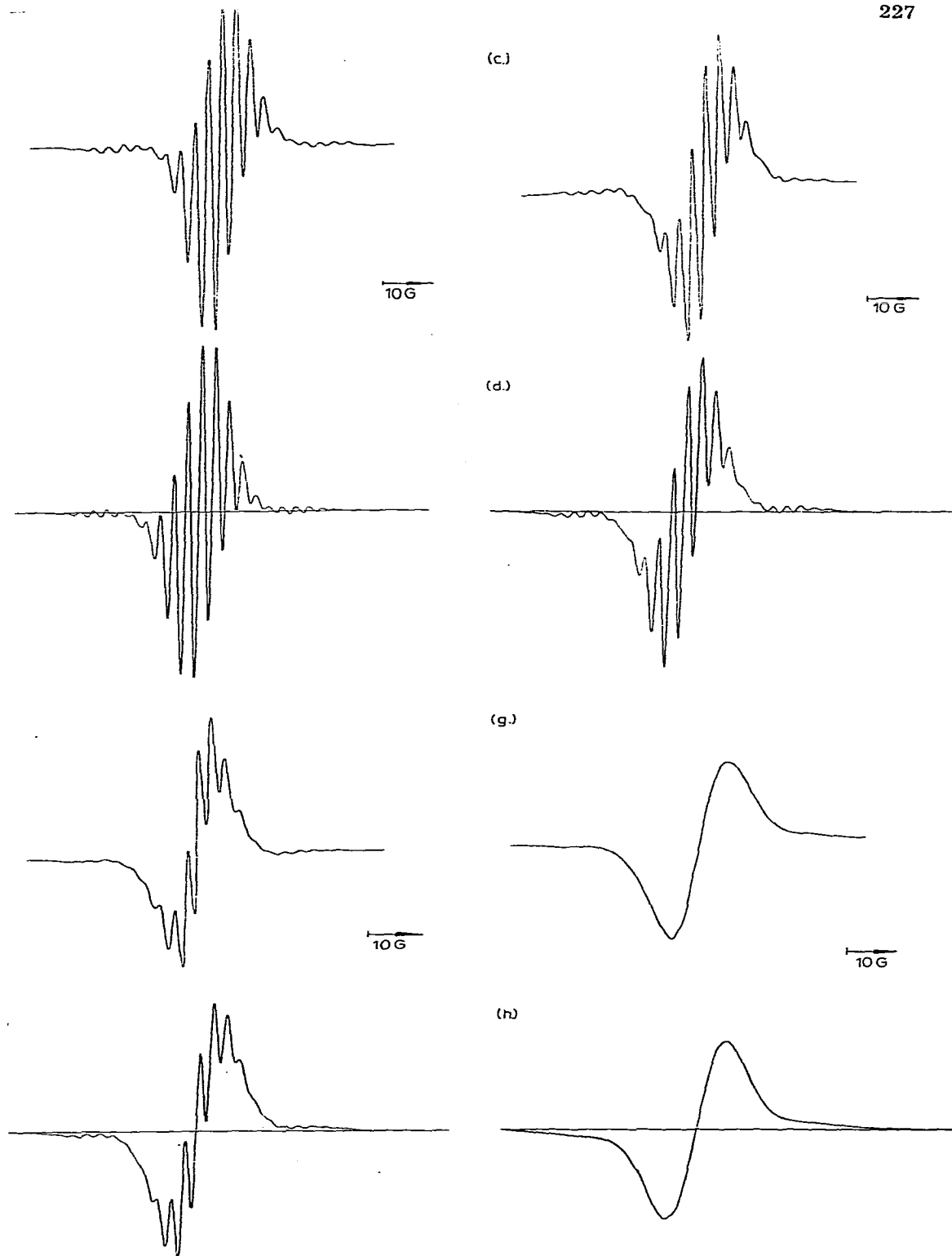
Fig. 1. ESR spectra of 5.4 \times 10^{-4} M (C_6H_5Cl)_2Cr^+ in DMSO (a) No added (C_6H_5Cl)_2Cr^0 ( 22^\circ C ). (b) Computer simulation. (c) Added \sim 4 \times 10^{-2} M (C_6H_5Cl)_2Cr^0 ( 22^\circ C ). (d) Computer simulation. (e) Added \sim 8 \times 10^{-2} M (C_6H_5Cl)_2Cr^0 ( 22^\circ C ). (f) Computer simulation. (g) Added \sim 2 \times 10^{-1} M (C_6H_5Cl)_2Cr^0 ( 22^\circ C ). (h) Computer simulation.
