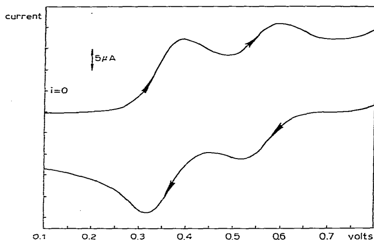
Fig. 3. Cyclic voltammogram of (\text{C}_6\text{H}_5\text{COOC}_2\text{H}_5)_2\text{Cr}^+ ( \sim 10^{-3} M ) at 25^\circ\text{C} in \text{DMSO}/0.1 M \text{ Bu}_4\text{NClO}_4 . The scan rate was 100 \text{ mV/sec} at \text{Pt} electrode.
