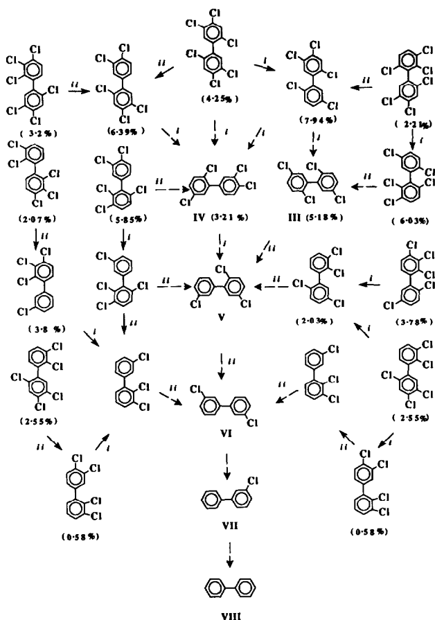
Fig. 3. Constructed dechlorination pathway of Aroclor 1254 of the 16 most abundant congeners of Aroclor 1254. (i) para elimination and (ii) ortho elimination. Percentage abundance (values in parentheses) are calculated using ref. 9. The structures 2,2',3',4,5-Cl 5 -BP, 2,3,3',4'-Cl 4 -BP and 2,3,3'-Cl 3 -BP are repeated for clarity.
