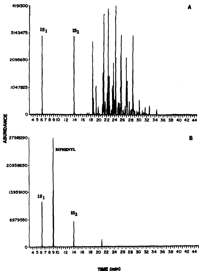
Fig. 1. GC/MS total ion chromatogram of Aroclor 1254 (0.20 g). (A) Before reaction; (B) after reaction with I (2.50 g)/Na (1.10 g) in THF (25 ml). The product is biphenyl. IS 1 = 1,2,3-Cl 3 -benzene and IS 2 = 4-Br-biphenyl as internal standards.
