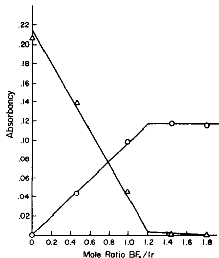
Figure 2. Infrared Titration of IrCOCl(P(C_6H_5)_3)_2 in C_6D_6 solution. \triangle 1968\text{ cm}^{-1} , \nu(CO) of parent complex; \circ 2067\text{ cm}^{-1} , \nu(CO) of adduct.
