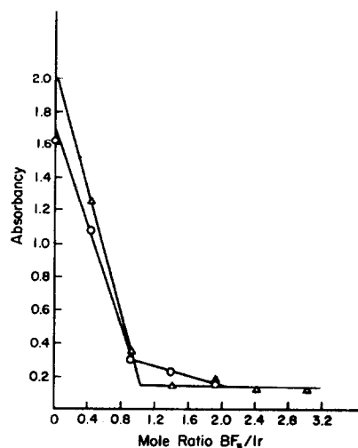
Figure 3. Spectrophotometric Titration of IrCOCl(P(C_6H_5)_3)_2 . \triangle 387\text{ nm} band; \circ 338\text{ nm} band.
