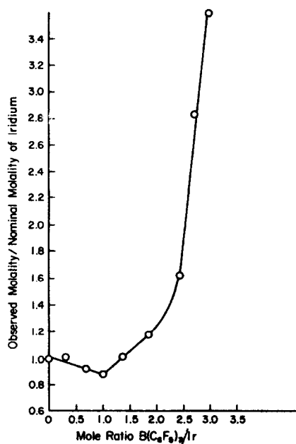
Figure 4. Cryoscopic Titration of \text{IrClCO}(\text{P}(\text{C}_2\text{H}_5)_2\text{C}_6\text{H}_5)_2 with \text{B}(\text{C}_6\text{F}_5)_3 in Benzene Solution.
