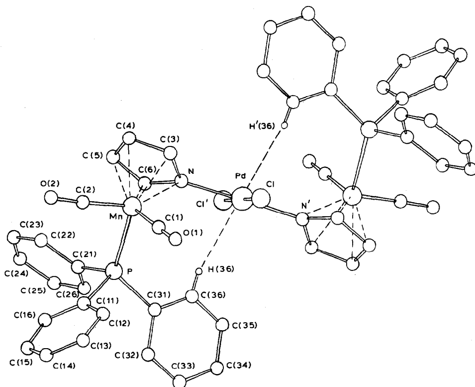
Fig. 1. Molecular structure of [(PPh_3)(CO)_2Mn(\eta^5-C_4H_4N)]_2PdCl_2 (III), including atomic numbering. The hydrogen atoms, except H(36), have been omitted.
