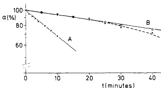
Figure 1. Relative specific activities of 2 (A) and 3 (B) ( 5 \times 10^{-3} M) as a function of time on irradiation ( \lambda = 313 nm) with \text{NaOCH}_3 (0.25 M) in MeOH: \times , uncorrected for concurrent reduction and nitrososubstitution; \circ , corrected.
