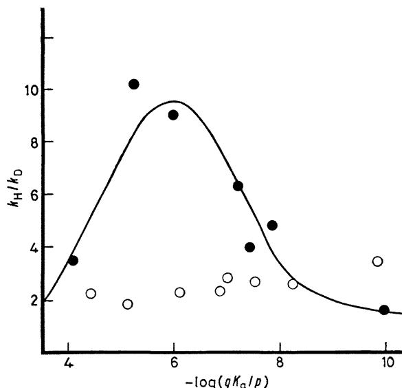
FIGURE. Kinetic isotope effects on nitramide decomposition [equation (2)] via the first reaction pathway catalysed by oxygen bases obtained in this study (○) ( B = RPO_3^{2-} ) compared with those reported in ref. 2 (●) ( B = ArO^- ).
