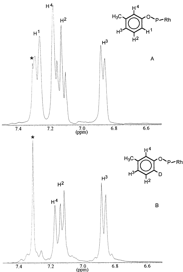
Fig. 4. ^1\text{H} -NMR spectra of \text{HRh}\{\text{P}(\text{O-3-CH}_3\text{C}_6\text{H}_4)_3\}_4 (A) and \text{DRh}\{\text{P}(\text{O-2-D, 3-CH}_3\text{C}_6\text{H}_3)_3\}_4 (B) in \text{C}_6\text{D}_6 in the phenyl proton region (* traces of \text{C}_6\text{H}_6 in \text{C}_6\text{D}_6 ).
