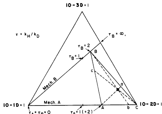
Figure 1. Tertiary component plot for products 10-1D, -2D, and -3D from mechanisms A, B, and C with variable k_{\text{H}}/k_{\text{D}} ( \tau ). The experimental point is 73% 10-2D, 18% 10-3D, and 9% 10-1D. This example assumes \tau_{\text{A}} = \tau_{\text{B}} = 2 .
