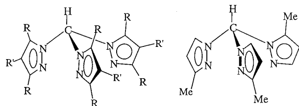
HC(pz) 3 CH: R = R' = H HC(4-Mepz) 3 : R = H, R' = Me HC(3,5-Me 2 pz) 3 : R = Me, R' = H HC(3,4,5-Me 3 pz) 3 : R = R' = Me
