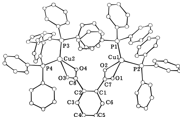
Figure 2. SCHAKAL drawing of complex 8 .
