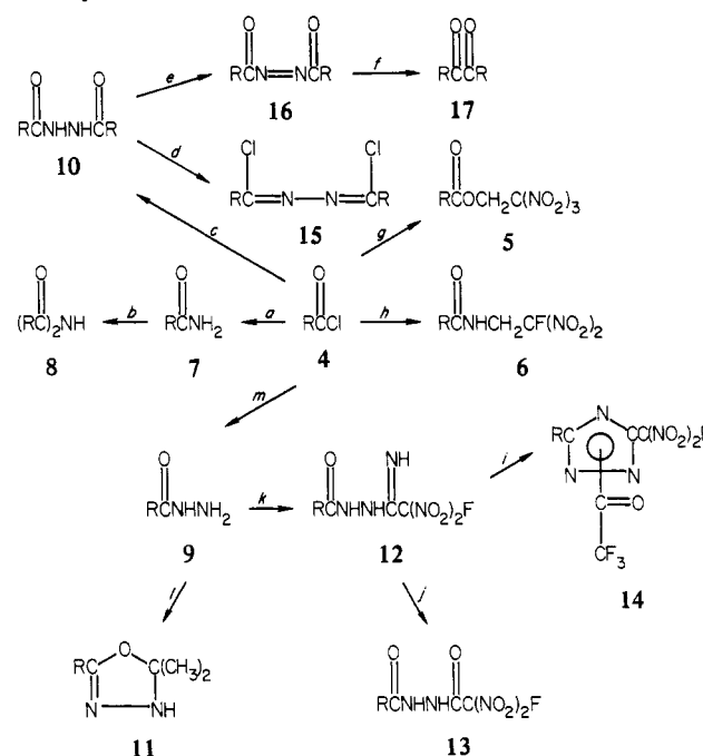
Scheme I. Derivatives of N,N -Bis(2-fluoro-2,2-dinitroethyl)-carbamyl Chloride
