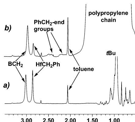
Figure 12. Propylene polymerization in a NMR tube using 14 as catalyst (a) before addition of propylene and (b) after 1 min of propylene bubbling. Conditions: \text{C}_6\text{D}_5\text{Br} , temperature 27 °C.
