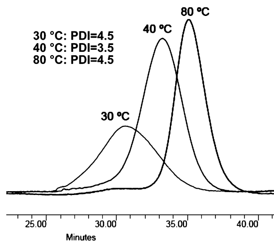
Figure 6. GPC curves of polyethylenes obtained with the catalyst 7/MAO at different polymerization temperatures: 30, 40, and 80 ^{\circ}\text{C} . PDI: molar mass distribution ( M_w/M_n ).
