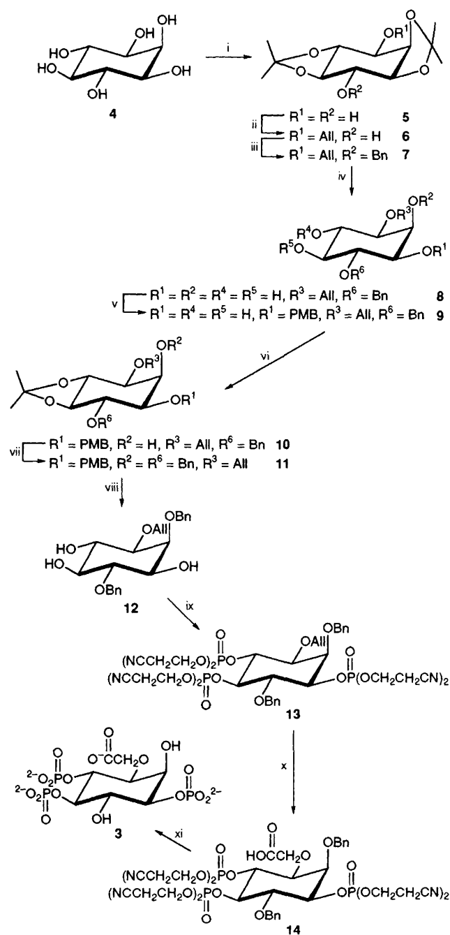
Scheme 1 Reagents and conditions: i, (a) MeC(MeO) 2 Me, PTSA, reflux, (b) BzCl, pyridine, (c) NaOH, reflux; ii, allyl bromide, BaO/Ba(OH) 2 ; iii, BnCl, NaH; iv, PTSA, ethyl acetate-acetone-water (9:9:1 v/v); v, (a) dibutyltin oxide, reflux, (b) CsF, ( p -MeO)BnCl; vi, 2-methoxypropene, PTSA; vii, BnCl, NaH; viii, M HCl, reflux; ix, Pr t 2 NP(OCH 2 CH 2 CN) 2 , tetrazole in CH 2 Cl 2 , (b) 70% Bu t OOH; x, NaIO 4 , RuCl 3 ·xH 2 O; xi, (a) Na/liq. NH 3 , (b) H 2 O. All compounds except 4 are racemic. All = allyl, PMB = p -methoxybenzyl, Bn = benzyl, PTSA = p -toluene sulfonic acid.
