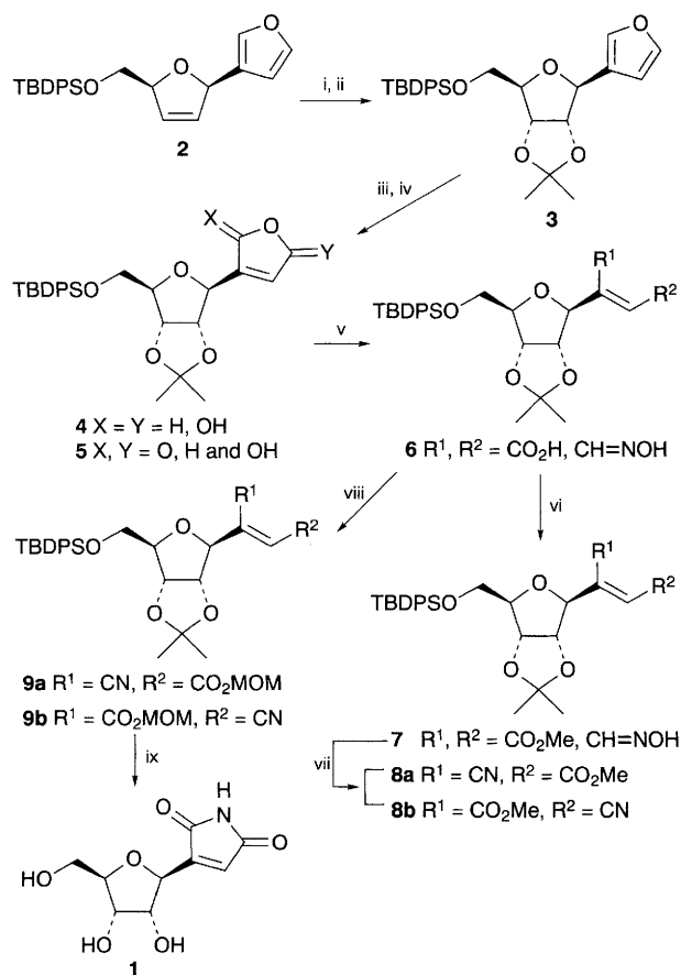
Scheme 1 Reagents and conditions: i, OsO 4 (cat.), NMO, aq. acetone, -20^\circ\text{C} ; ii, p -TsOH (cat.), acetone, room temp.; iii, Br 2 (2 equiv.), K 2 CO 3 (0.5 equiv.), THF–H 2 O (5:1), 0^\circ\text{C} ; iv, CrO 3 on Celite (3 equiv.), CH 2 Cl 2 –Et 2 O (3:1), 0^\circ\text{C} ; v, HONH 2 ·HCl, pyridine–MeOH (1:1), room temp.; vi, CH 2 N 2 , Et 2 O, 0^\circ\text{C} ; vii, MeSO 2 Cl, Pr 2 NEt, CH 2 Cl 2 , -20 to 0^\circ\text{C} ; viii, MOMCl, Pr 2 NEt, CH 2 Cl 2 , -30 to -20^\circ\text{C} , then MeSO 2 Cl, -30 to 0^\circ\text{C} ; ix, CF 3 CO 2 H, (CF 3 CO) 2 O, 45^\circ\text{C} , then H 2 O, room temp.
