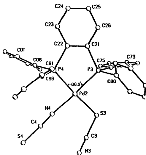
Fig. 6. Molecular structure of [\text{Pd}(\text{dpbz})(\text{NCS})(\text{SCN})] .
