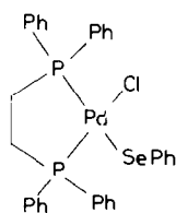
Fig. 2. Suggested structure for complex V.
