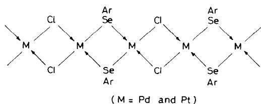
Fig. 1. Proposed structure for complex [MCl(SeAr)] n (I).
