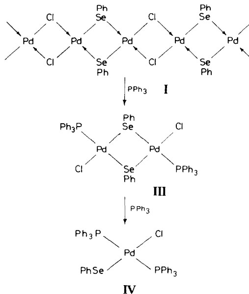
Scheme 1. Suggested mechanism for the formation of complex IV from complex I and PPh 3 (excess).
