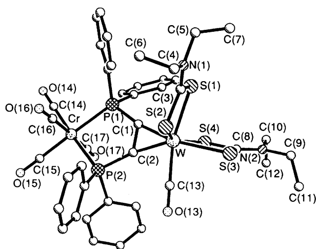
Fig. 1 The molecular structure of [W(CO) 4 ](Ph 2 PC≡CPh) 2 Cr(CO) 4 (S 2 CNEt 2 ) 2 2 showing the atom labelling system
