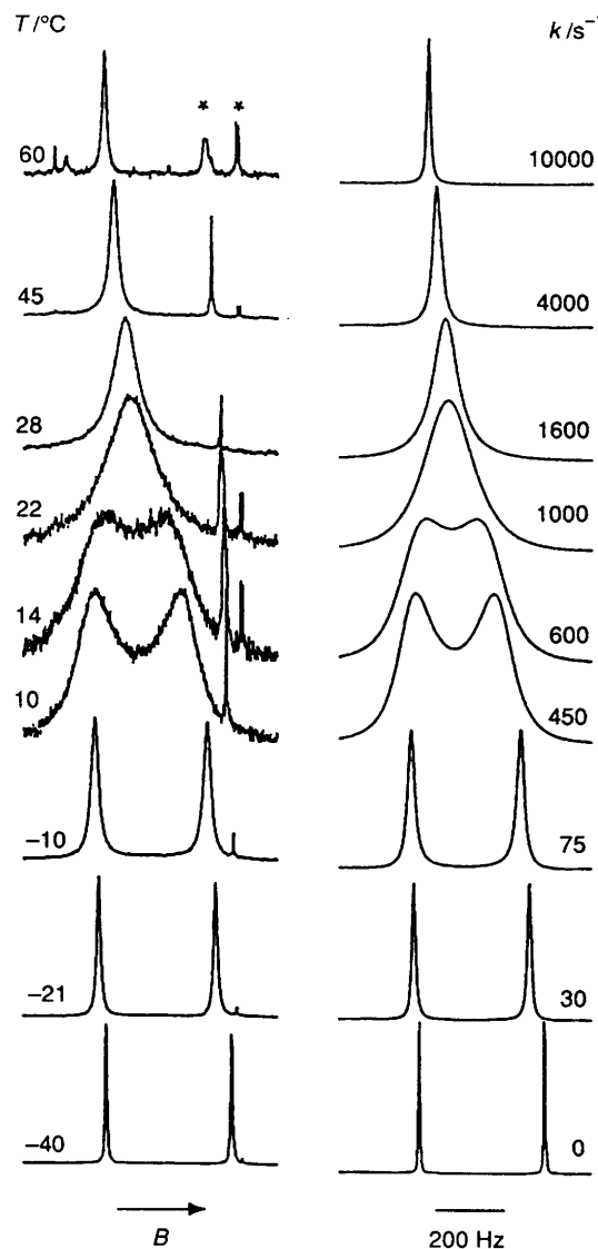
Fig. 3 Variable-temperature ^{31}\text{P}\{-^1\text{H}\} NMR spectra of complex [\text{W}(\text{CO})\{(\text{Ph}_2\text{PC}\equiv\text{CPh}_2)\text{Mo}(\text{CO})_4\}(\text{S}_2\text{CNEt}_2)_2] 3 and their computer syntheses; the asterisk indicates an impurity
