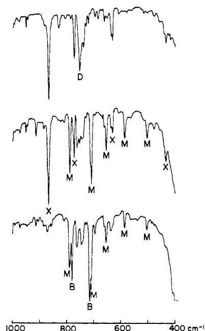
Figure 4. Top: Infrared spectrum (in transmittance) of o -xylxylene ( 6a ) obtained upon irradiation (>514 nm, 820 min; >470 nm, 4196 min) of o -tolyl diazomethane ( 2a ) matrix isolated in argon at 15 K. D, residual diazo compound. Middle: Infrared spectrum of the product mixture obtained upon irradiation (>416 nm, 1301 min) of o -tolyl diazomethane ( 2a ) matrix isolated in argon at 15 K. X, o -xylxylene ( 6a ); M, 1-methylcycloheptatetraene ( 12a ). Bottom: Infrared spectrum showing the disappearance of o -xylxylene ( 6a ) and appearance of benzocyclobutene ( 7a ) upon irradiation (>267 nm, 1938 min) of the sample shown immediately above. B, benzocyclobutene ( 7a ); M, 1-methylcycloheptatetraene ( 12a ).
