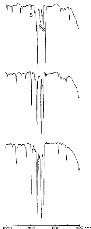
Figure 6. Top: Infrared spectrum (in transmittance) of 2,2,2-trideuterio-1-phenylethylidene ( 8b ) formed upon irradiation (>470 nm, 1532 min) of 2,2,2-trideuterio-1-phenyldiazoethane ( 1b ) matrix isolated in argon at 15 K. S, \alpha,\beta,\beta -trideuteriostyrene ( 5b ). Middle: Infrared spectrum of \alpha,\beta,\beta -trideuteriostyrene ( 5b ) formed upon irradiation (>420 nm, 20 min) of the sample shown immediately above. Bottom: Infrared spectrum of \alpha,\beta,\beta -trideuteriostyrene ( 5b ) formed upon flash vacuum thermolysis (390 °C) of 2,2,2-trideuterio-1-phenyldiazoethane ( 1b ) followed by cocondensation of the pyrolyzate with argon.
