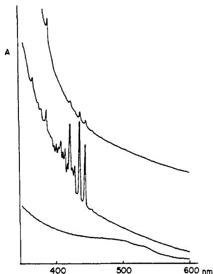
Figure 1. UV/visible absorption spectra obtained upon irradiation of p -tolyl-diazomethane ( 4a ) matrix isolated in argon at 15 K. Bottom: 4a prior to irradiation. Middle: Formation of p -tolylmethylene ( 11a ) (>470 nm, 3960 min). Top: Disappearance of 11a (>416 nm; 285 min).
