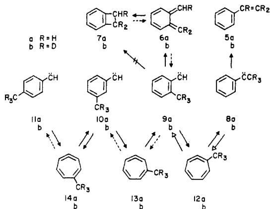
Scheme IV
