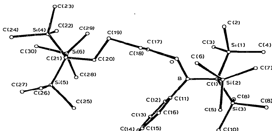
Fig. 1. Structure of (\text{Me}_3\text{Si})_3\text{CB(Ph)[O(CH}_2)_4\text{C(SiMe}_3)_3] .
