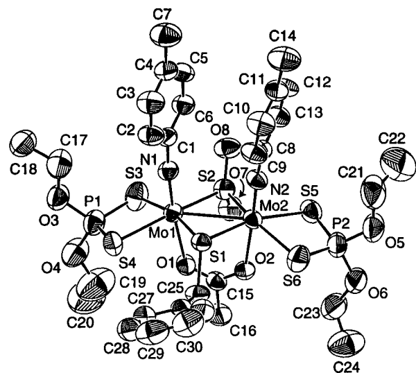
Figure 3. ORTEP view of [\text{Mo}_2(\text{NT0})_2(\text{S}_2\text{P}(\text{OEt})_2)_2(\text{O}_2\text{CMe})(\text{SBz})-(\text{SO}_2)] , 4 ( \text{R} = \text{Bz} ).
