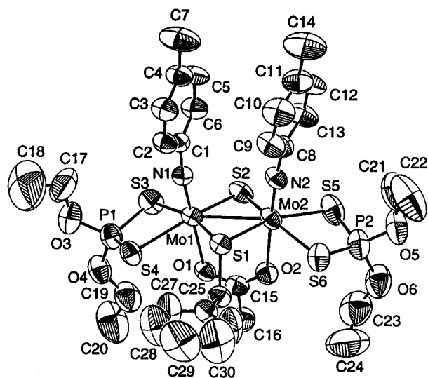
Figure 1. ORTEP view of [\text{Mo}_2(\text{NT0})_2(\text{S}_2\text{P}(\text{OEt})_2)_2(\text{O}_2\text{CMe})(\text{SBz})-(\text{S})] , 2 ( \text{R} = \text{Bz} ).
