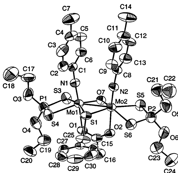
Figure 4. ORTEP view of [\text{Mo}_2(\text{NTo})_2(\text{S}_2\text{P}(\text{OEt})_2)_2(\text{O}_2\text{CMe})(\text{SBz})(\text{O})] , 5 ( \text{R} = \text{Bz} ).
