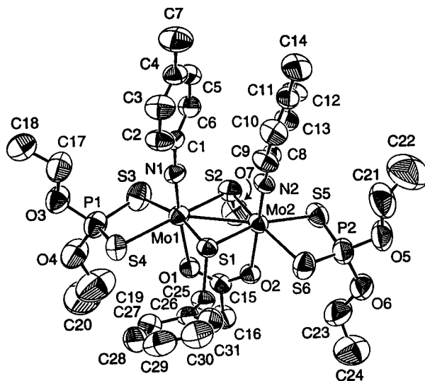
Figure 2. ORTEP view of [\text{Mo}_2(\text{NT0})_2(\text{S}_2\text{P}(\text{OEt})_2)_2(\text{O}_2\text{CMe})(\text{SBz})-(\text{SO})] , 3 ( \text{R} = \text{Bz} ). This view clearly shows the pyramidity of S(2).
