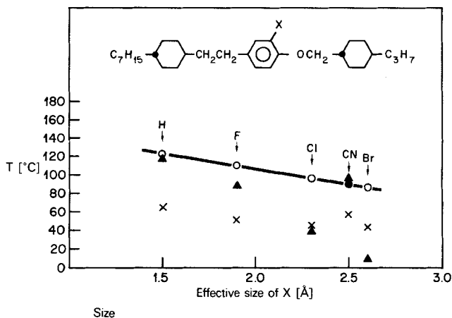
Figure. Plot of the transition temperatures vs. the size of the lateral substituent (X) of the ether formulated ( X , crystal-smectic/nematic transition; \blacktriangle , smectic-nematic/isotropic liquid transition; \circ , enantiotropic nematic-isotropic liquid transition; \bullet , monotropic nematic-isotropic liquid transition)
