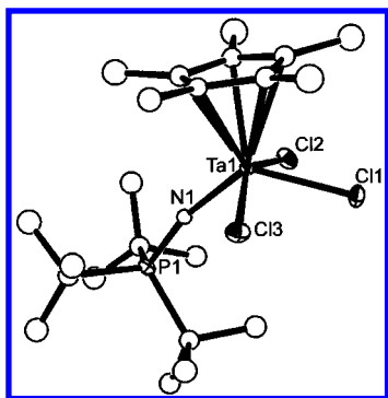
Figure 1. ORTEP drawings of 1 , 30% thermal ellipsoids are shown. Hydrogen atoms have been omitted for clarity. Selected bond distances (Å) and angles (deg): Ta(1)–N(1) 1.870(13), Ta(1)–Cl(1) 2.437(5), Ta(1)–Cl(2) 2.440(5), Ta(1)–Cl(3) 2.449(5), P(1)–N(1) 1.585(14), N(1)–Ta(1)–Cl(1) 127.8(4), N(1)–Ta(1)–Cl(2) 89.4(4), N(1)–Ta(1)–Cl(3) 87.0(4), Cl(1)–Ta(1)–Cl(2) 78.7(2), Cl(1)–Ta(1)–Cl(3) 78.8(2), Cl(2)–Ta(1)–Cl(3) 148.22(19), P(1)–N(1)–Ta(1) 165.7(8).
