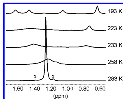
Figure 2. The tert -butyl group resonances region of the ^1\text{H} NMR spectrum of 1 as a function of temperature.
