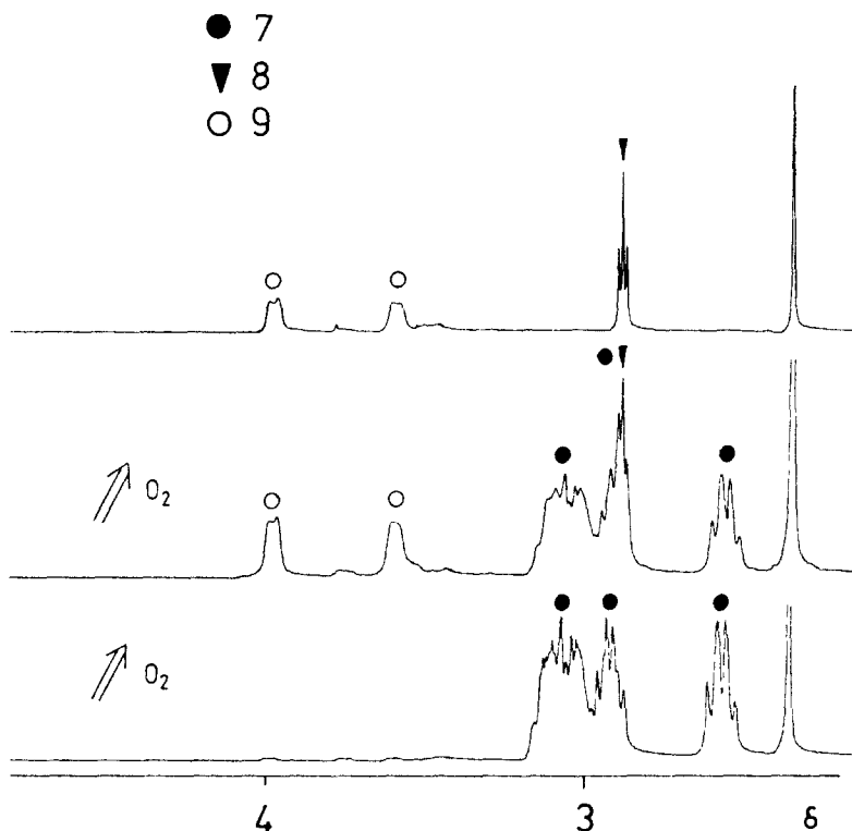
Fig. 4. Monitoring of the reaction between complex 7 and dioxygen in \text{CD}_2\text{Cl}_2 (i) (a) ^{31}\text{P} NMR spectrum of starting material (b) at intermediate time and (c) on completion of reaction; (ii) (a) ^1\text{H} NMR spectrum of starting material (b) at intermediate times and (c) on completion of reaction.
