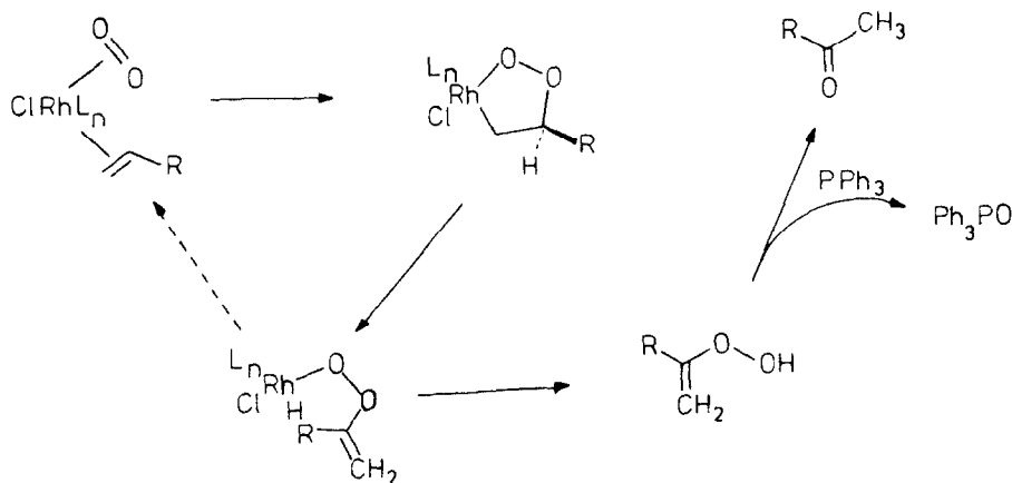
SCHEME 1. Olefin oxidation mechanism involving a metalladioxacyclopentane
