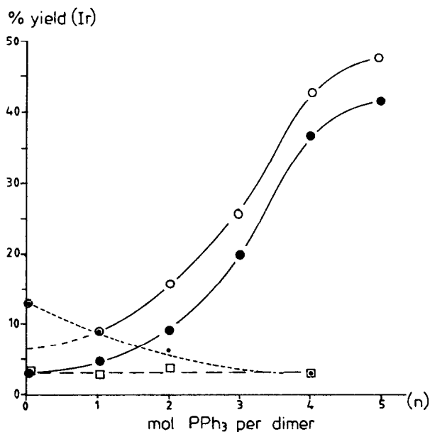
Fig. 3. Effect of added triphenylphosphine on the oxidation of styrene (280 mM) in the presence of [(PhCH=CH_2)_2IrCl]_2 (28 mM) under an oxygen atmosphere. Acetophenone, 2 h, ●; 10 h, ○; Benzaldehyde 2 h □; 10 h, •.
