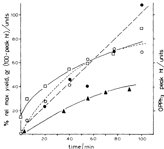
Fig. 2. Monitoring of the oxidation of oct-1-ene and decomposition of \text{ClIr}(\text{PPh}_3)_3(\text{O}_2) in \text{CH}_2\text{Cl}_2 (54 mM) thus: (a) Decay of complex under argon, ^{31}\text{P} NMR \blacktriangle ; (b) Decay of complex under argon in the presence of oct-1-ene (271 mM) \circ ; (c) experiment b, monitoring the formation of octan-2-one by GLC \bullet ; (d) experiment b, monitoring formation of \text{PPh}_3\text{O} by ^{31}\text{P} NMR, \square .
