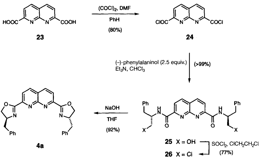
Scheme 5
