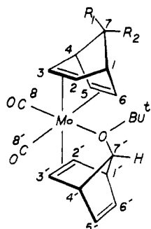
10a: \text{R}_1 = \text{O}-t\text{-Bu} ; \text{R}_2 = \text{H} b: \text{R}_1 = \text{H} ; \text{R}_2 = \text{O}-t\text{-Bu}
