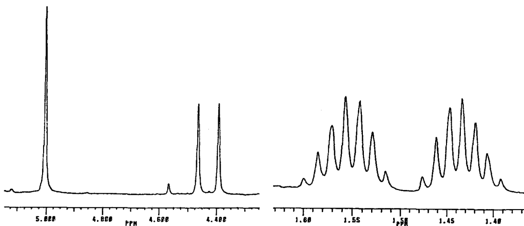
Figure 6. Portion of 1 H-NMR spectra of reaction of the chiral derivative (39) with (R)-(-)-2-butanol. The peak at ~5 ppm is the C-11 H of the starting material, while the peaks at ~4.40 and 4.45 ppm are due to the C-11 H of the ether products. No attempt was made to assign absolute configurations.
