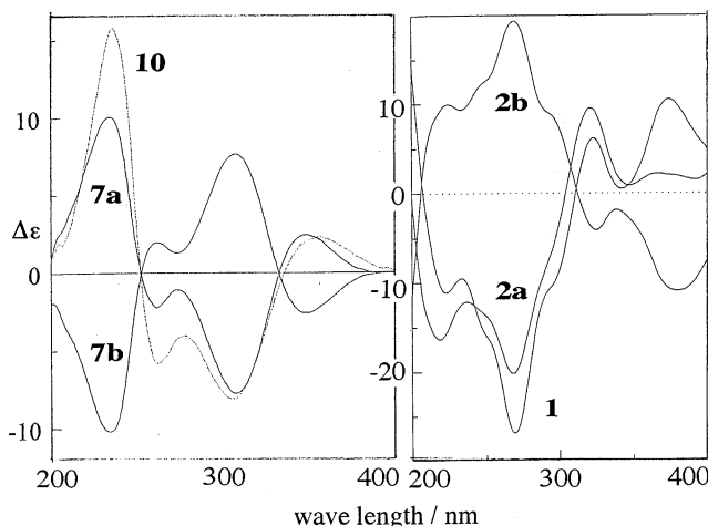
Figure 2. CD spectra of (+)- and (-)-model compounds 7a, b and 2a, b , and C-β-D-glucopyranosylcyclohexadienone 10 and carthamin 1 .
