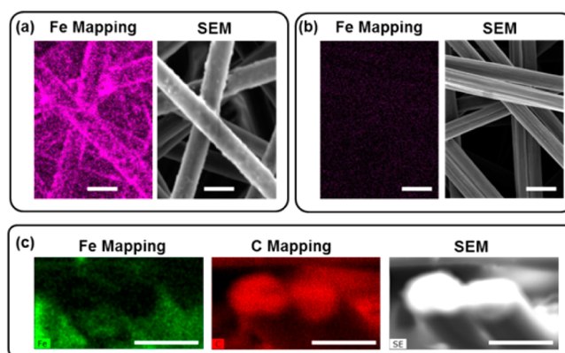
Figure 4. EDS elemental mapping. (a) Fe mapping and corresponding SEM image of PVF-coated CFs (10 min deposition). (b) Fe mapping and corresponding SEM image of unmodified CFs. (c) Fe mapping, C mapping, and corresponding SEM image of the cross section of cryo-fractured PVF-coated CFs (10 min deposition). Scale bar: 10 \mu\text{m} .
