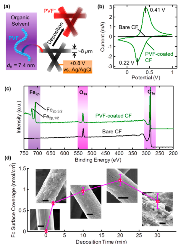
Figure 2. Preparation of PVF/CF hybrids. (a) Schematics of oxidation-induced conformational deposition of PVF onto CFs. (b) CVs of a bare and a PVF-coated CF matrix. Scan rate: 50 mV/s. Electrolyte: 0.5 M NaClO 4 . (c) XPS spectra of a bare and a PVF-coated CF matrix. (d) Ferrocene surface coverage versus deposition time. Insets: corresponding SEM images of the specimens. Scale bar: 2 μm.
