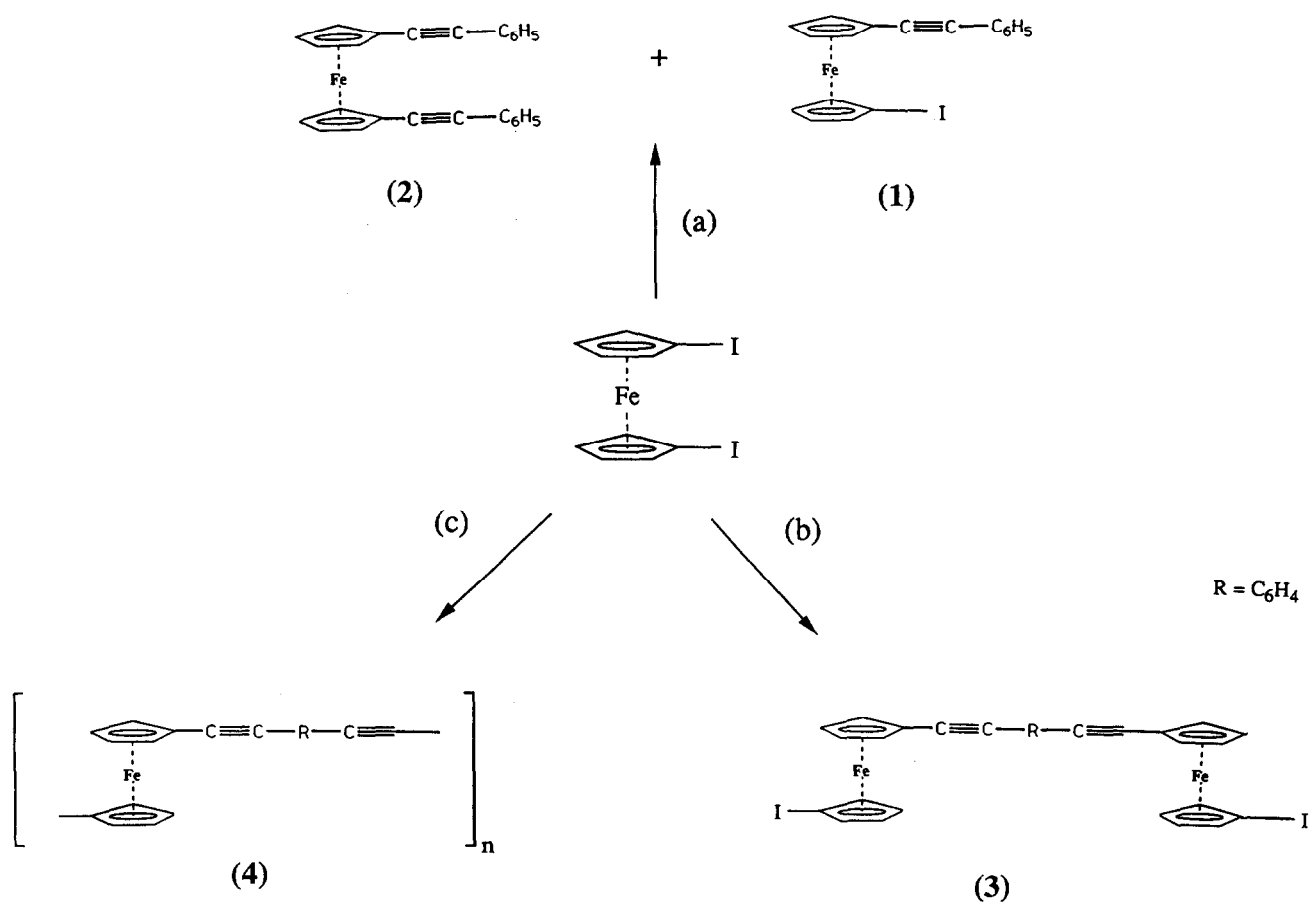
Scheme 1. (a) 2.5 equiv. \text{Me}_3\text{SnC}\equiv\text{CPh} + [\text{Pd}(\text{PPh}_3)_4] (2 mole-%); (b) 0.3 equiv. \text{Me}_3\text{SnC}\equiv\text{CC}_6\text{H}_4\text{C}\equiv\text{CSnMe}_3 + [\text{Pd}(\text{PPh}_3)_4] (2 mole-%); (c) 1.0 equiv. \text{Me}_3\text{SnC}\equiv\text{CC}_6\text{H}_4\text{C}\equiv\text{CSnMe}_3 + [\text{Pd}(\text{PPh}_3)_4] (2 mole-%).
