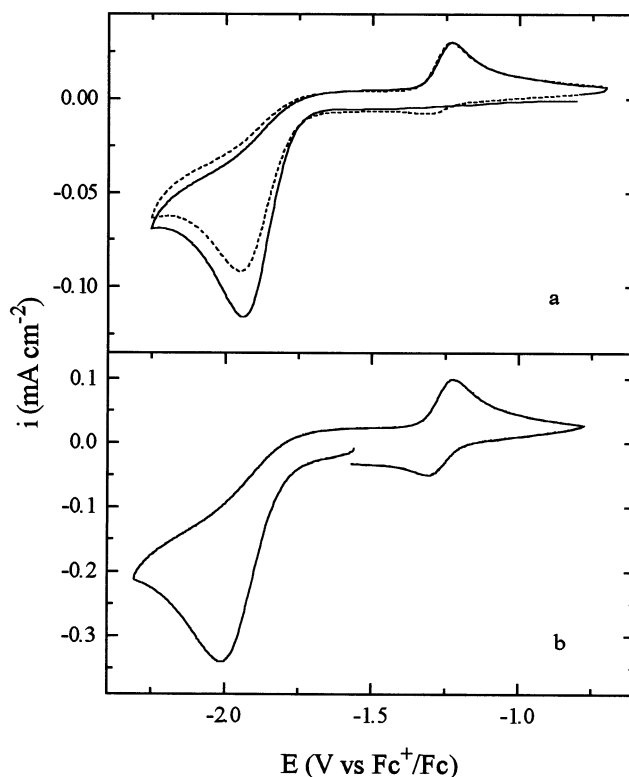
Fig. 5. Cyclic voltammograms for the reduction of a 8.5 \times 10^{-4} \text{ M} solution of 4 in PC containing 0.2 \text{ M TBAPF}_6 at 25^\circ\text{C} . The first (—) and second (---) scans are shown in a. The sweep rate is 0.1 \text{ Vs}^{-1} in a, and 1 \text{ Vs}^{-1} in b. An asterisk indicates the start of a cycle.
