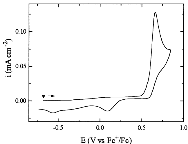
Fig. 3. Cyclic voltammogram for the oxidation of a 1.4 \times 10^{-3} \text{ M} solution of 3 in PC containing 0.2 \text{ M TBAPF}_6 at 0.1 \text{ Vs}^{-1} and 25^\circ\text{C} . An asterisk indicates the start of the run.
