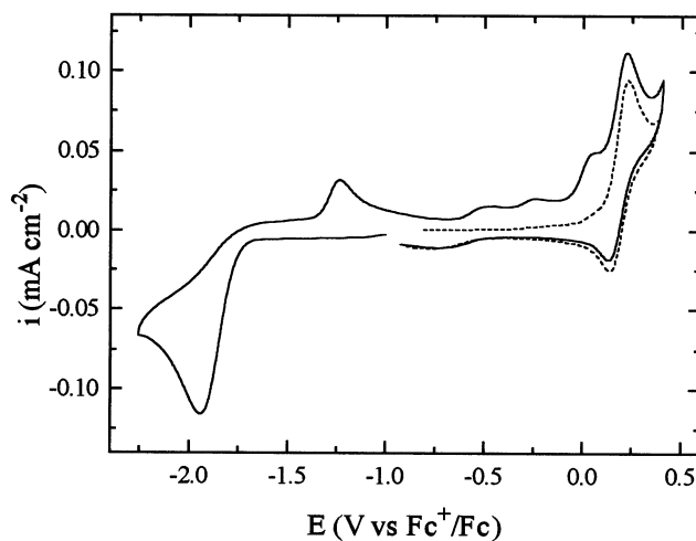
Fig. 6. Cyclic voltammogram of a 8.5 \times 10^{-4} \text{ M} solution of 4 in PC containing 0.2 \text{ M TBAPF}_6 at 0.1 \text{ Vs}^{-1} and 25^\circ\text{C} . Scans started at ca. -1.0 \text{ V} in the cathodic direction (—) and in the anodic direction (---).
