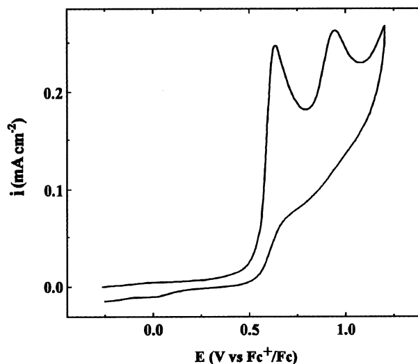
Fig. 4. Cyclic voltammogram for the oxidation of a 1.5 \times 10^{-3} \text{ M} solution of 1 in DCE containing 0.2 \text{ M TBAPF}_6 at 0.1 \text{ Vs}^{-1} and 25^\circ\text{C} . An asterisk indicates the start of the run.
