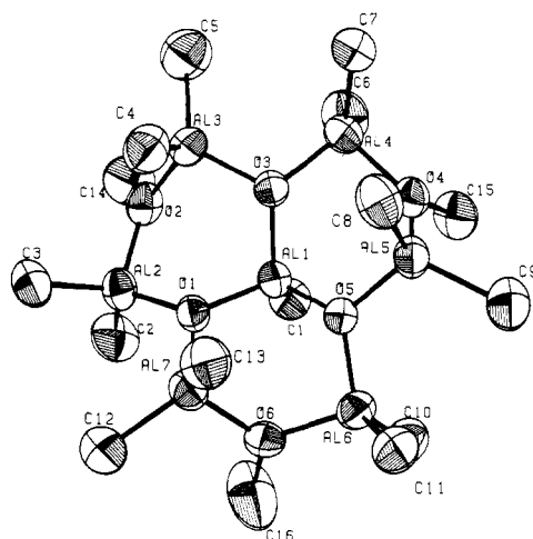
Figure 1. [\text{Al}_7\text{O}_6\text{Me}_{16}]^- anion with numbering scheme for \text{K}[\text{Al}_7\text{O}_6\text{Me}_{16}]\cdot\text{C}_6\text{H}_6 . The atoms are represented by their 50% probability ellipsoids for thermal motion.
