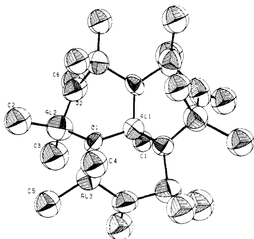
Figure 2. [\text{Al}_7\text{O}_6\text{Me}_{16}]^- anion for \text{Cs}[\text{Al}_7\text{O}_6\text{Me}_{16}]\cdot 3\text{C}_6\text{H}_5\text{Me} . The anion contains a crystallographic threefold axis.
