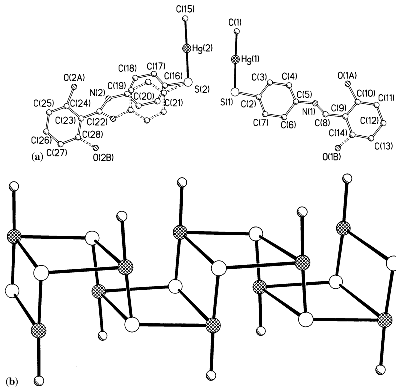
Fig. 5. The structure of [MeHg(4-SC 6 H 4 N=CHC 6 H 4 OH)] ( 8 ): (a) the asymmetric unit without H atoms, showing the atom numbering; (b) the core of the ladder structure common to this and compounds 5 and 7 .
