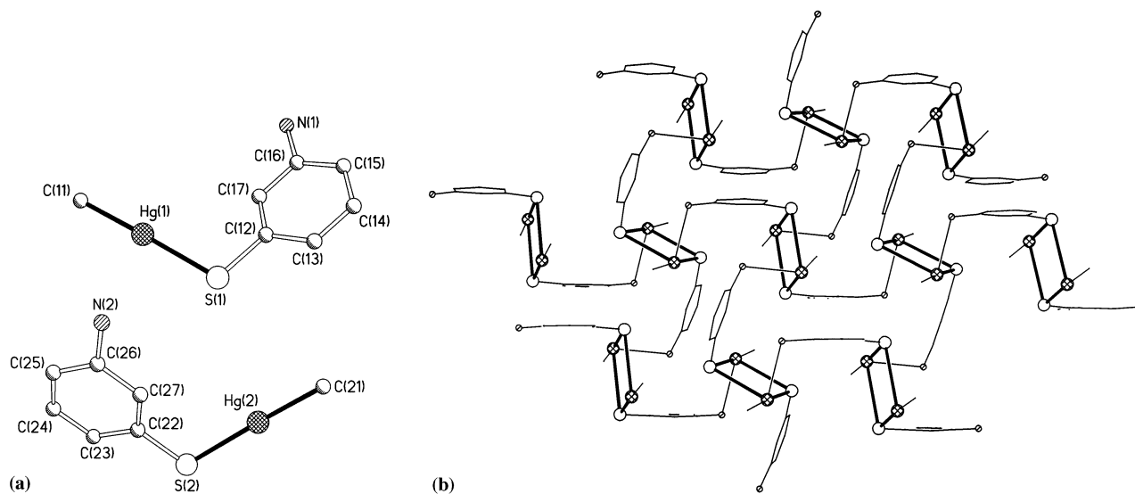
Fig. 2. The structure of [\text{MeHg}(3\text{-SC}_6\text{H}_4\text{NH}_2)_2] ( 3 ): (a) the asymmetric unit without H atoms, showing the atom numbering; (b) part of the sheet network resulting from \text{Hg}\cdots\text{S} and \text{Hg}\cdots\text{N} secondary interactions.
