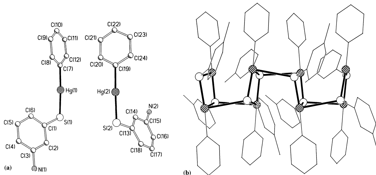
Fig. 3. The structure of [PhHg(3-SC 6 H 4 NH 2 ) 2 ] ( 5 ): (a) the asymmetric unit without H atoms, showing the atom numbering; (b) a section of the zig-zag ladder formed through Hg...S interactions.
