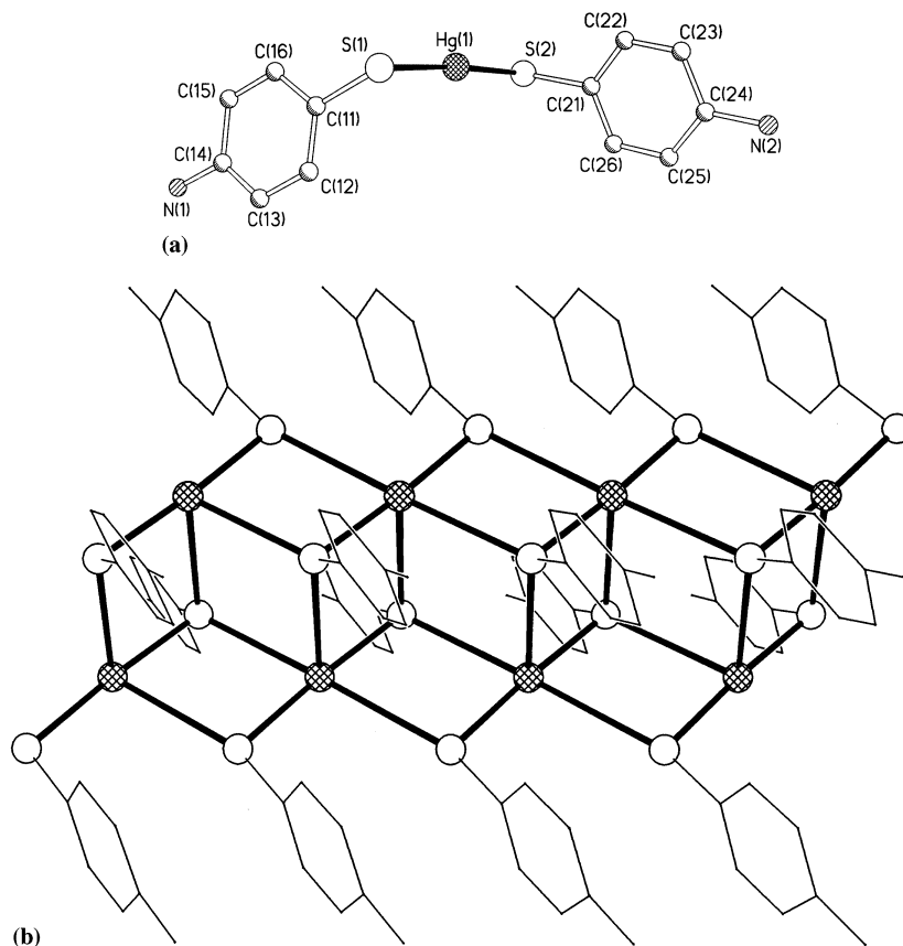
Fig. 1. The structure of [\text{Hg}(4\text{-SC}_6\text{H}_4\text{NH}_2)_2] ( 2 ): (a) the asymmetric unit without H atoms, showing atom numbering; (b) a section of the polymeric chain of linked incomplete \text{Hg}_3\text{S}_4 cubanes.
