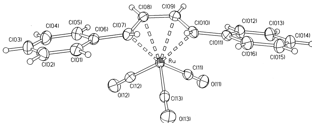
Fig. 1. Molecular structure of [\text{Ru}(\text{CO})_3\{(\text{E},\text{E})\text{-1,4-diphenylbuta-1,3-diene}\}] 3 .
