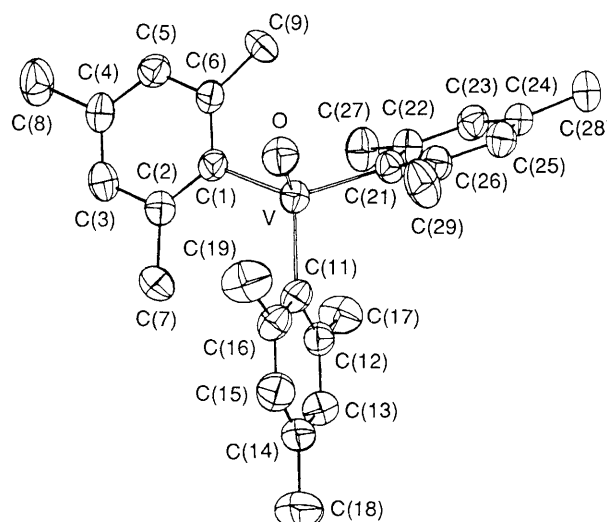
Fig. 1 An ORTEP drawing for complex 2 . Bond distances (Å) and angles ( ^\circ ): V-O 1.578(4), V-C(1) 2.078(4), V-C(11) 2.022(4), V-C(21) 2.079(3), C(11)-V-C(21) 108.5(2), C(1)-V-C(21) 122.3(2), C(1)-V-C(11) 116.3(2), O-V-C(21) 102.4(2), O-V-C(11) 105.0(2), O-V-C(1) 99.2(2).
