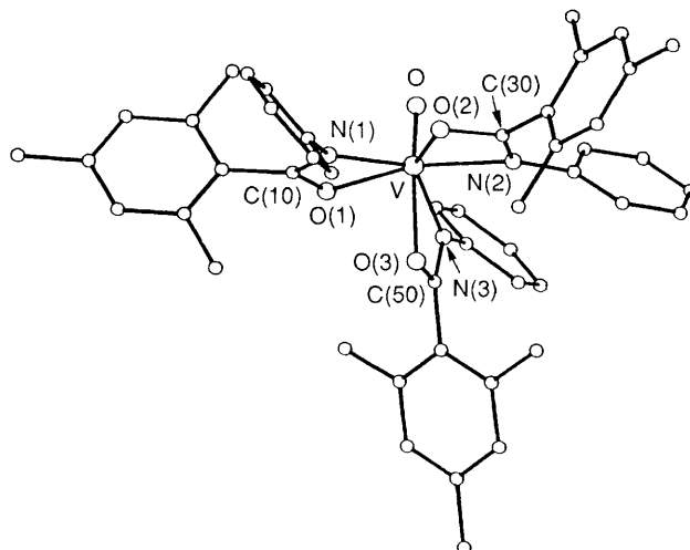
Fig. 2 A PLUTO drawing for complex 7 . Bond distances (Å) and angles ( ^\circ ): V-O 1.594(3), V-O(1) 2.152(3), V-N(1) 2.053(3), V-O(2) 2.011(3), V-N(2) 2.112(3), V-O(3) 2.197(3), V-N(3) 2.040(3), C(30)-V-C(50) 101.7(1), C(10)-V-C(50) 96.4(1), C(10)-V-C(30) 139.0(1), O(4)-V-C(10) 94.8(1), O(4)-V-C(30) 97.4(1), O(4)-V-C(50) 134.9(1).
