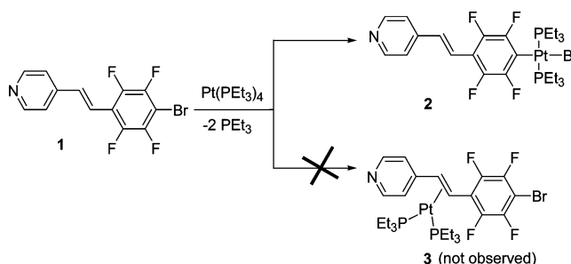
Scheme 1. Direct Generation of Complex 2 without Parallel Formation and/or Intermediacy of the Postulated Complex 3; Ar–Br Oxidative Addition Is Kinetically Preferred over \eta^2 -C=C Coordination
